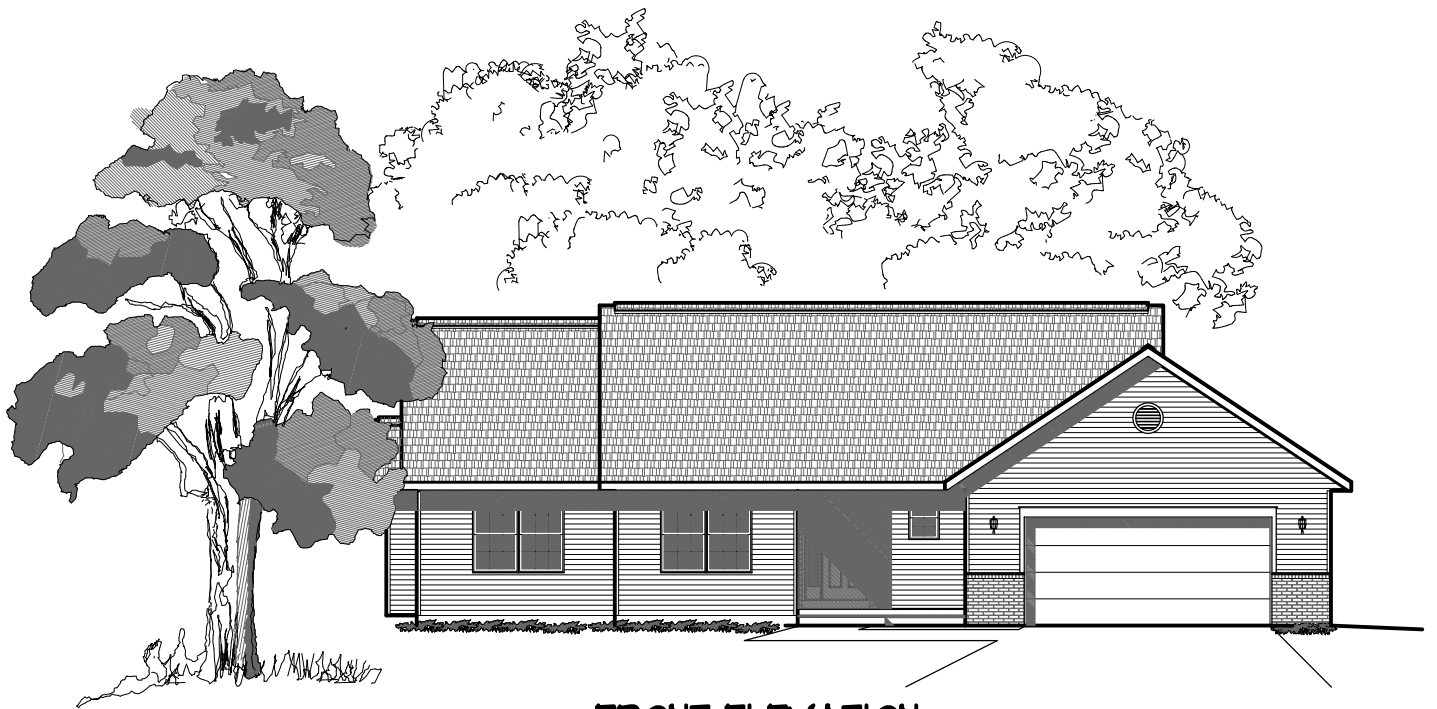
FRONT ELEVATION
